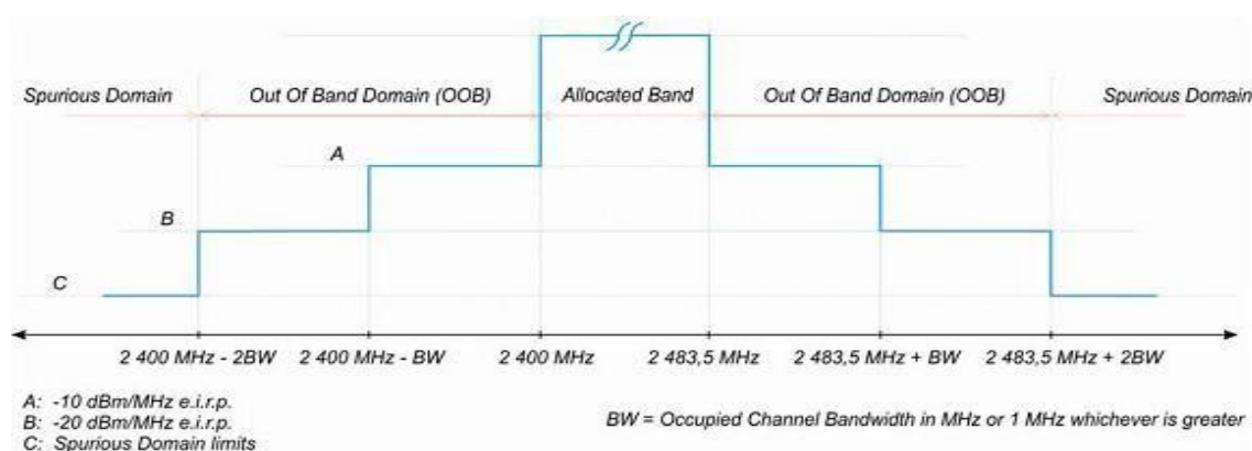
Figure 1: Transmit mask
